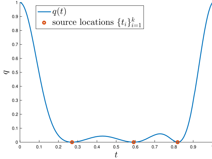
Fig. 3. Example of dual certificate q(t) required in Lemma 14. Here, we have k = 3 and t_1 = 0.27 , t_2 = 0.59 and t_3 = 0.82 .
