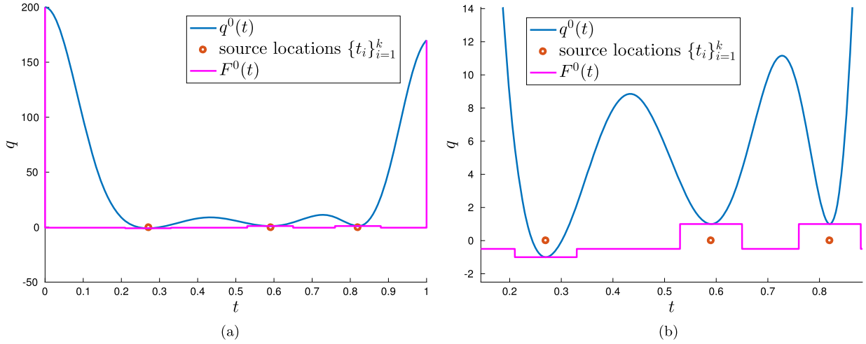
Fig. 5. Example of dual certificate q^0(t) that satisfies the conditions in Lemma 17 where the window function is the Gaussian kernel \phi(t) = e^{-t^2/\sigma^2} . We take k = 3 and t_i \in \{0.27, 0.59, 0.82\} and the function F^0(t) for the sign pattern \pi^0 = \{-1, 1, 1\} such that q^0(t) \geq F^0(t) . For the Gaussian kernel, the existence of q^\pi(t) for any sign pattern \pi guarantees the existence of q^0(t) in Lemma 17.
