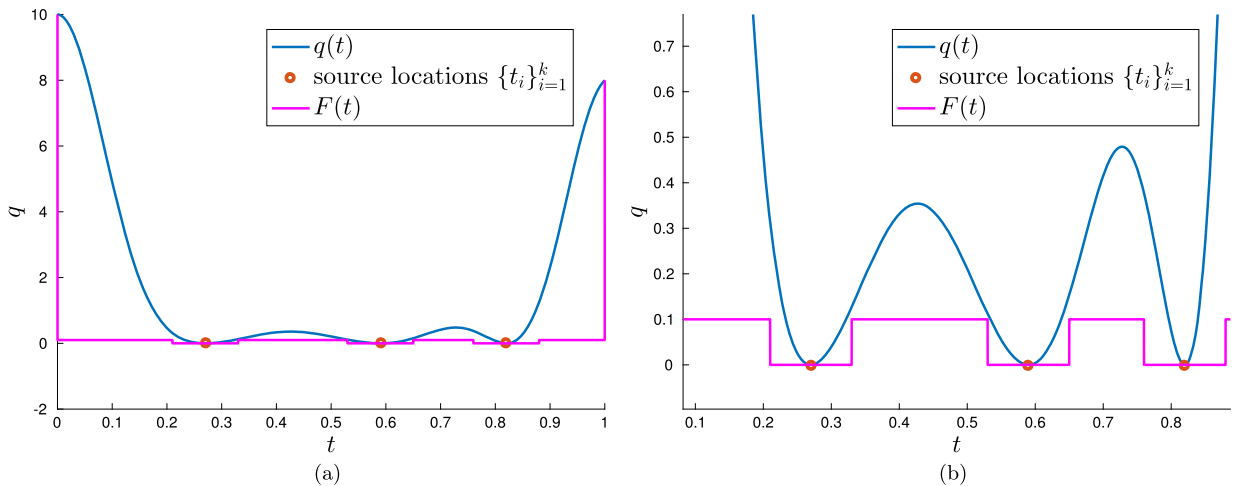
Fig. 4. Example of dual certificate q(t) that satisfies the conditions in Lemma 16 where the window function is the Gaussian kernel \phi(t) = e^{-t^2/\sigma^2} . We take k = 3 and t_i \in \{0.27, 0.59, 0.82\} and the function F(t) such that q(t) \geq F(t) .
