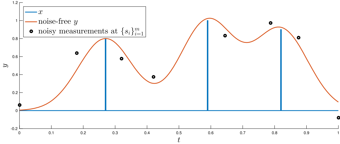
Fig. 1. Example of discrete measure x and measurements where \phi_j(t) = \phi(t - s_j) for s_j \in S and the Gaussian kernel \phi(t) = e^{-\frac{t^2}{\sigma^2}} . (For interpretation of the colours in the figure(s), the reader is referred to the web version of this article.)
